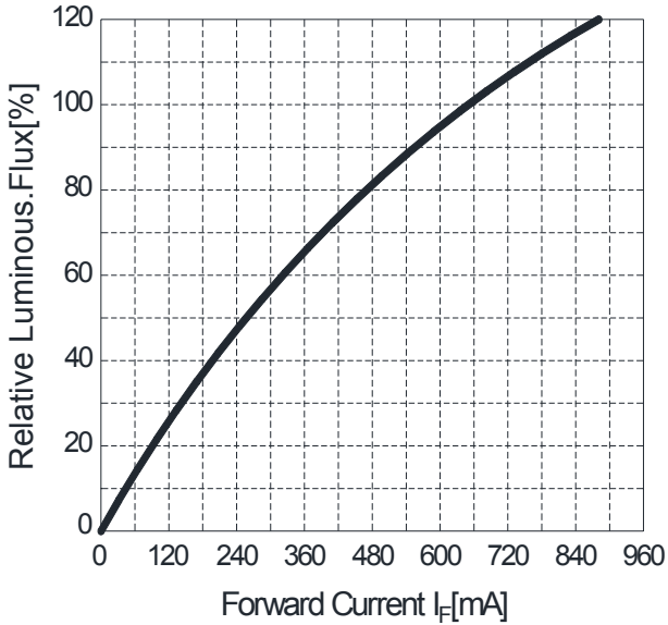
Relative Luminous.Flux( T_c=25^{\circ}C ) vs.Forward Current
