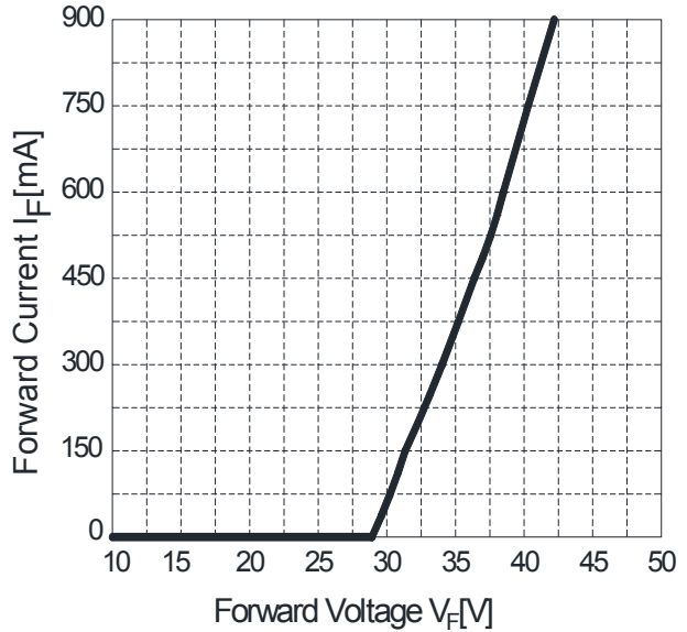
Forward Current( T_c=25^{\circ}C ) vs.Forward Voltage
