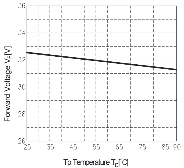
Forward Voltage (@640mA) vs. T_p Temperature
