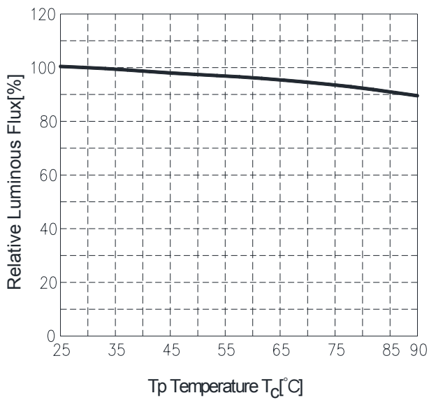
Relative Luminous Flux(@640mA) vs. T_p Temperature
