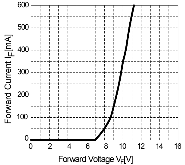
Forward Current( T_c=25^\circ\text{C} ) vs.Forward Voltage
